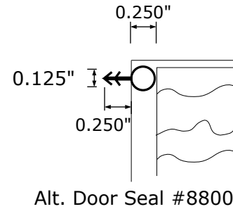
•Mortised Door Seal #8054N Detail (Top View):
