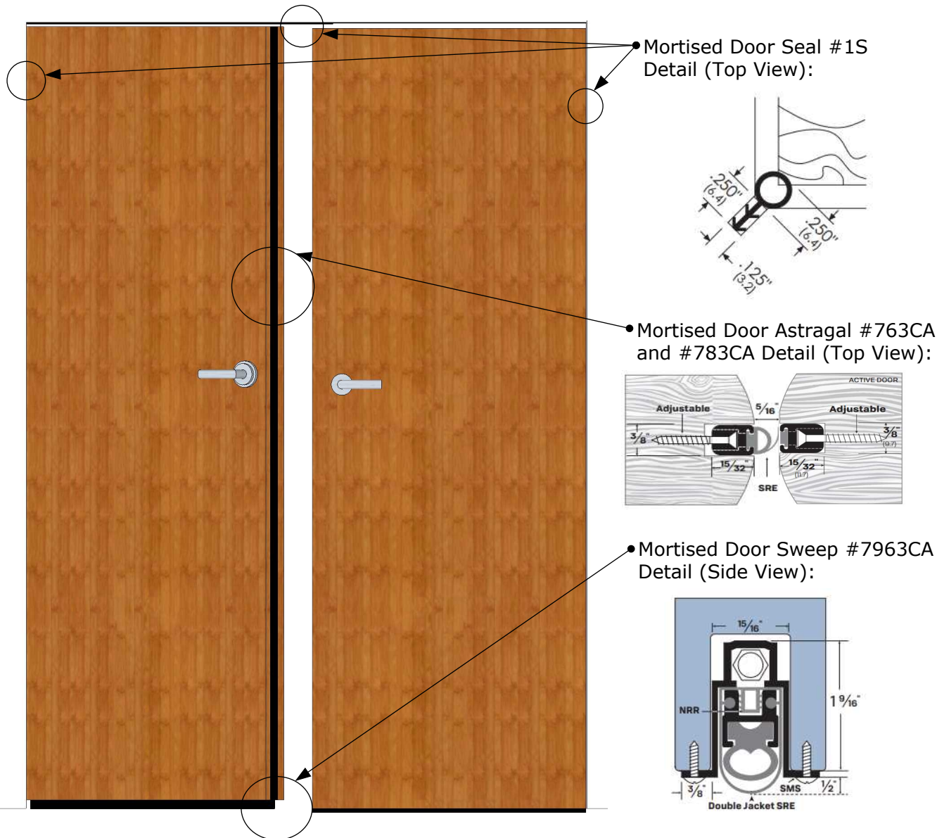
Double Door Seal Detail - #1s Perimeter Seal, #763CA and #783CA Astragal #7963CA Sweep
