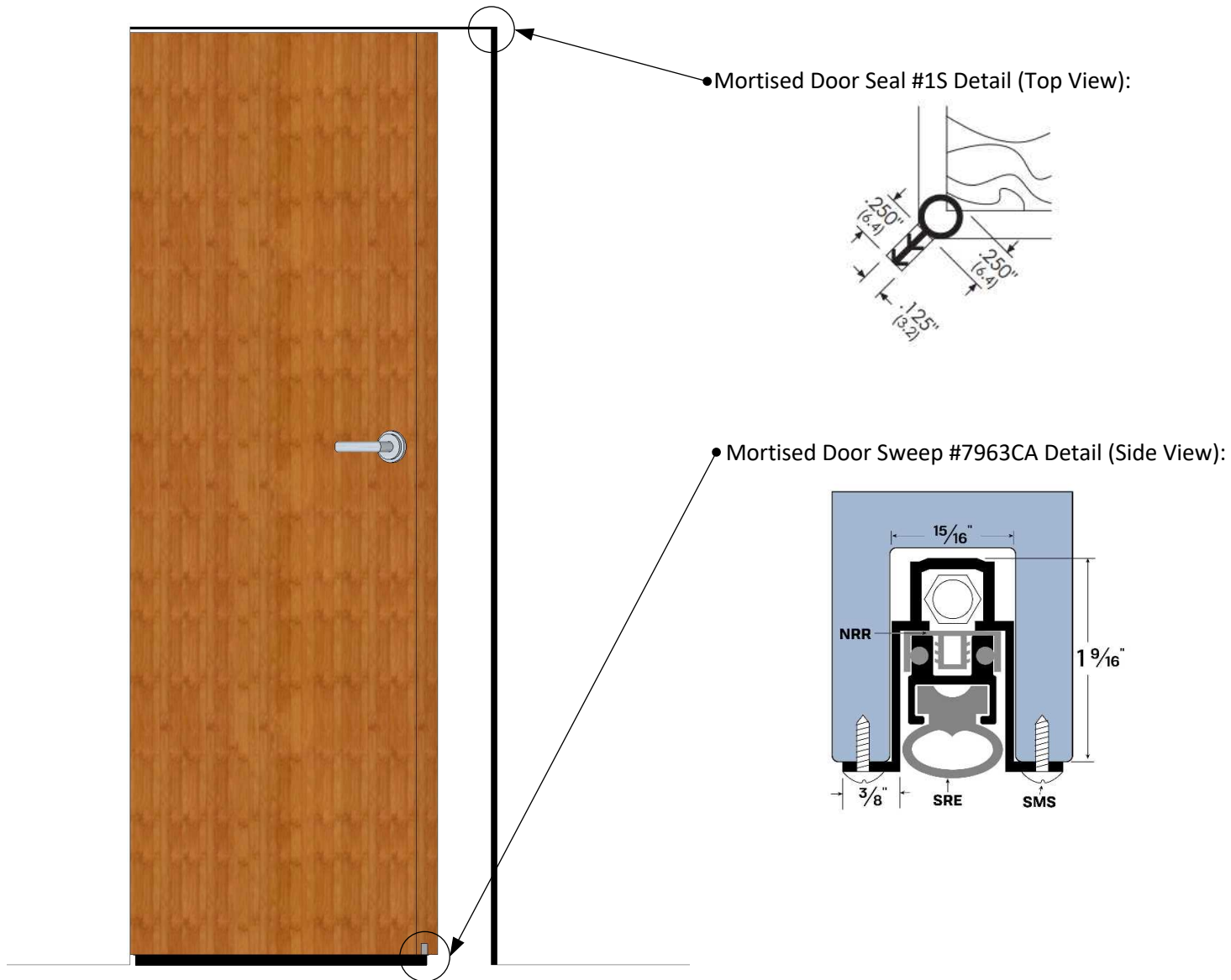
Single Leaf Door Seal Detail - #1S Seal, #7963CA Sweep
